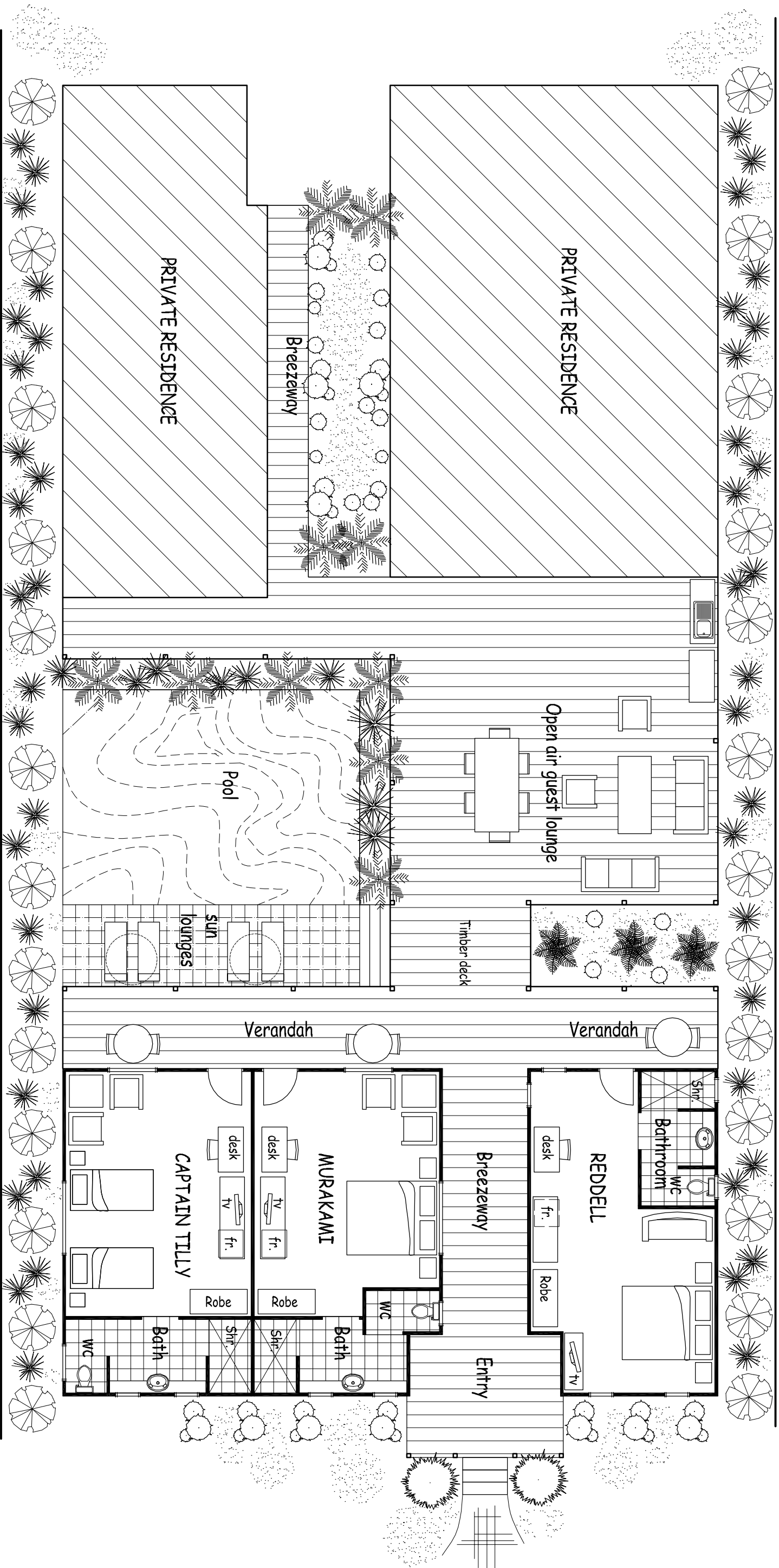
ACCOMMODATION PLAN
